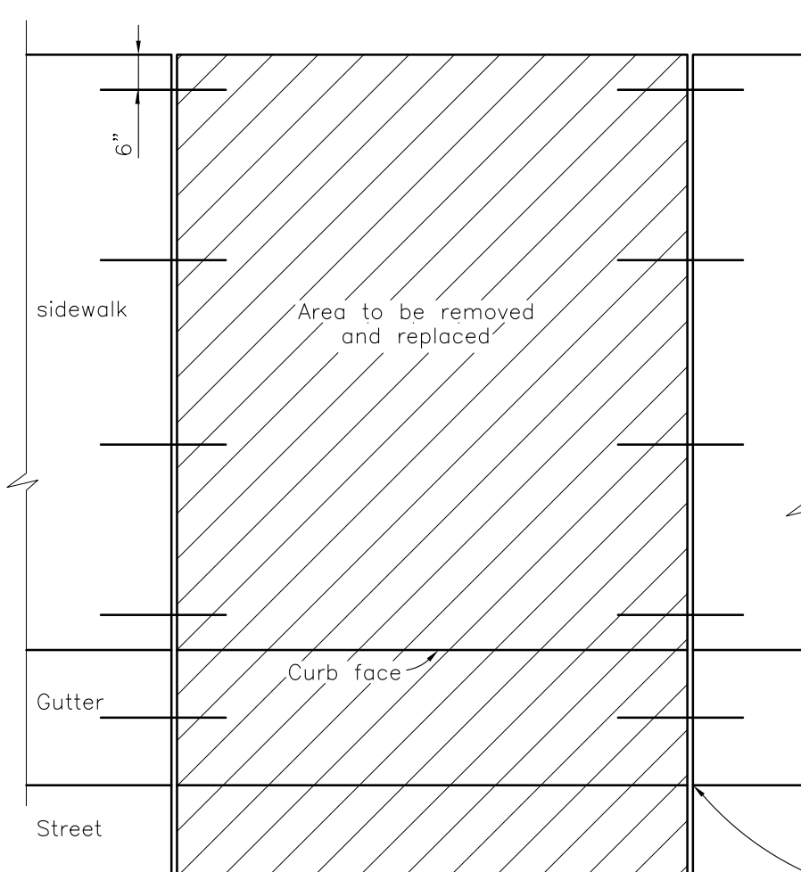
SIDEWALK SECTION
