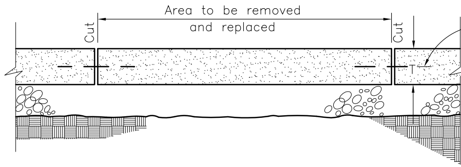
SIDEWALK SECTION
